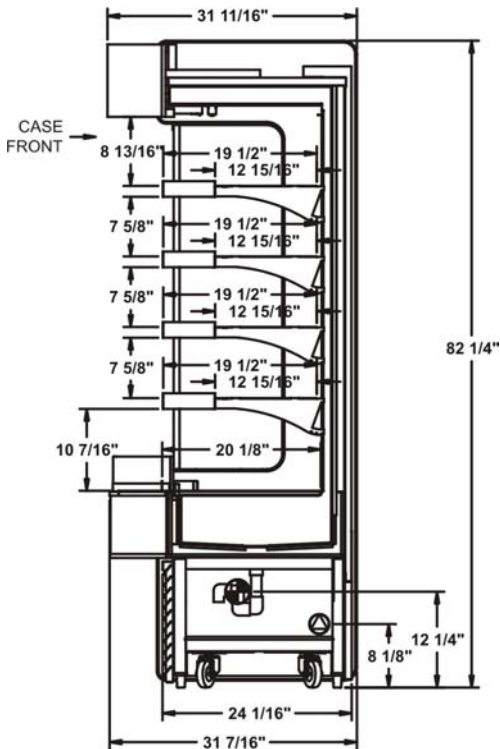
Curved front Option
