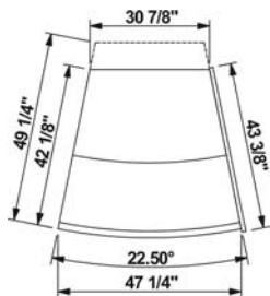
GHDSSX2 PLAN VIEW
