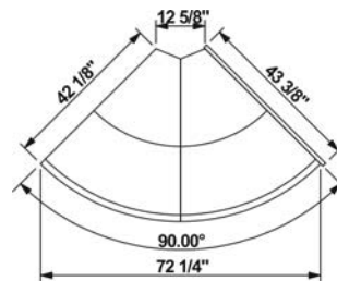
GHDSSX9 PLAN VIEW
