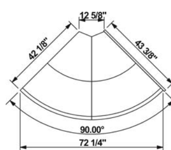
GMBSX9 PLAN VIEW
