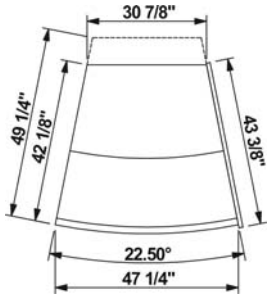
GMBSX2 PLAN VIEW
