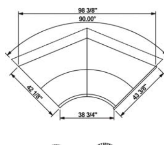
GMBSN9 PLAN VIEW
