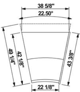
GMBSN2 PLAN VIEW
