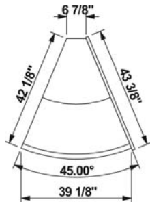
GMBSX4 PLAN VIEW
