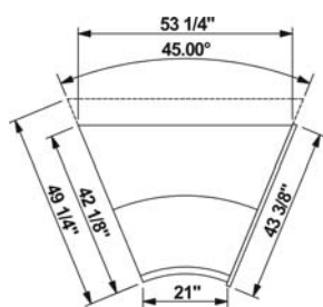
GMGN4 PLAN VIEW
