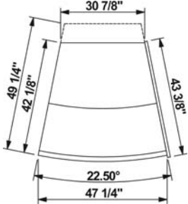
GMGX2 PLAN VIEW
