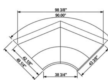
GMGN9 PLAN VIEW
