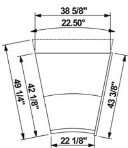
GMGN2 PLAN VIEW
