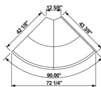
GMGX9 PLAN VIEW
