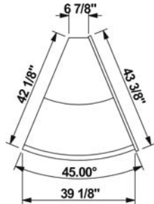
GMGX4 PLAN VIEW
