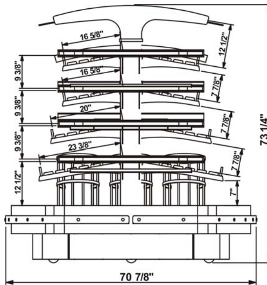
HV.4534B SIDE VIEW
