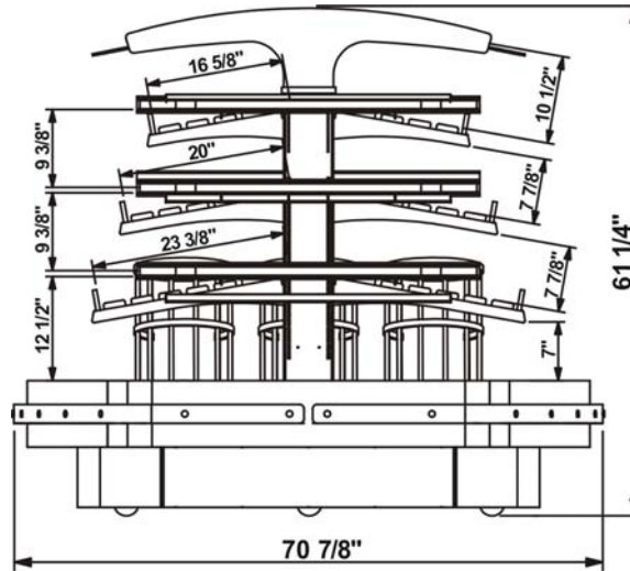
Standard HV.4534A SIDE VIEW
