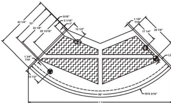
Plan View - FRCX90
