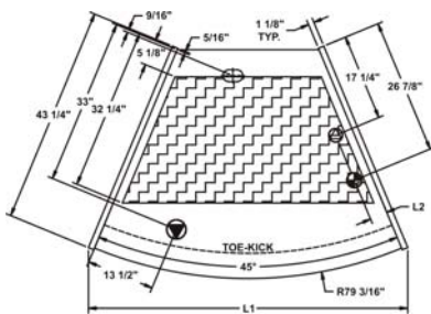
Plan View - FRCX90
