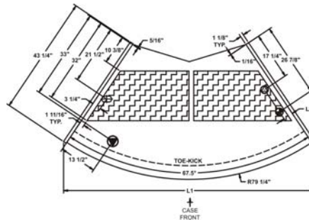
Plan View - FRCX67
