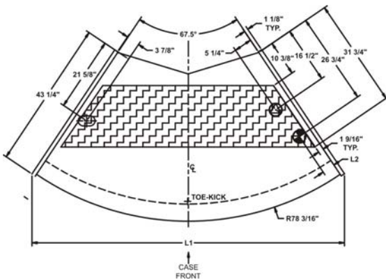
Plan View - F3CX
