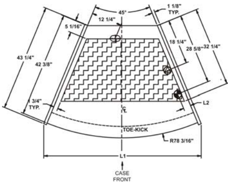
Plan View - F2CX
